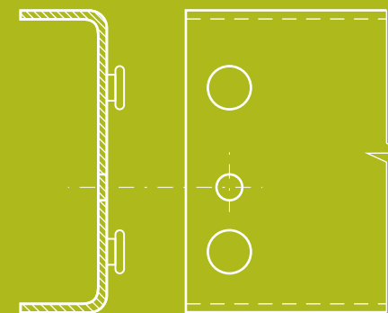
Heavy Rivet beam profile
